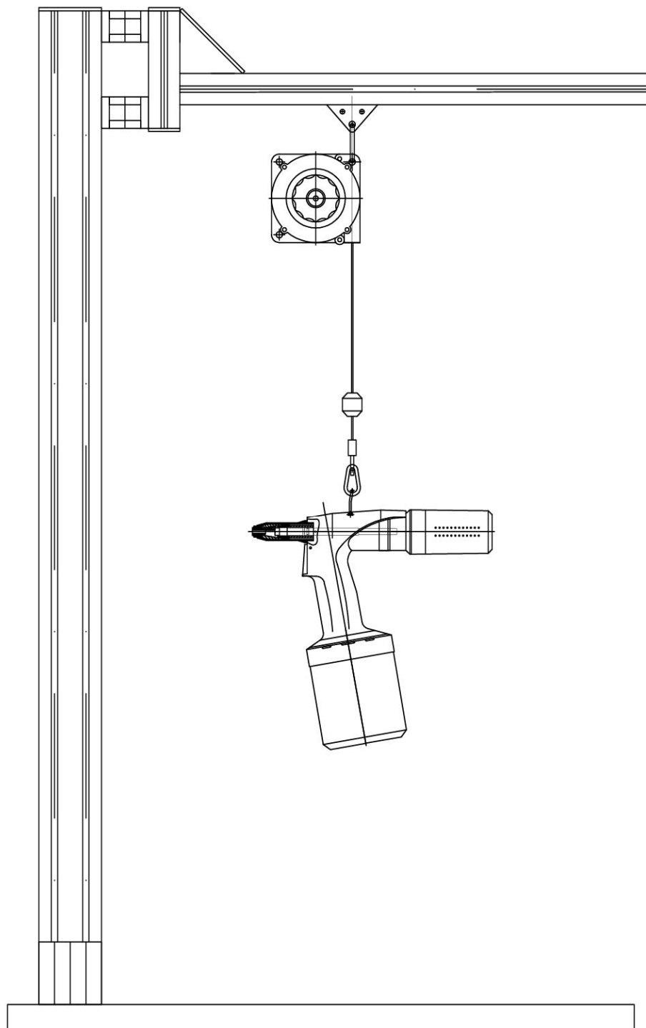
Tool holder with swivel arm and rivet tool AP3
