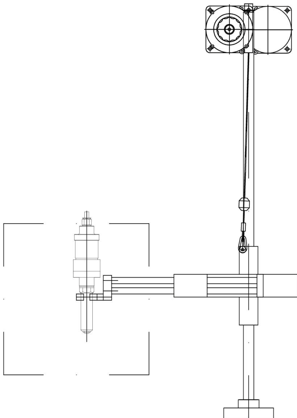
Tool holder with linear unit and rivet tool D7-10
