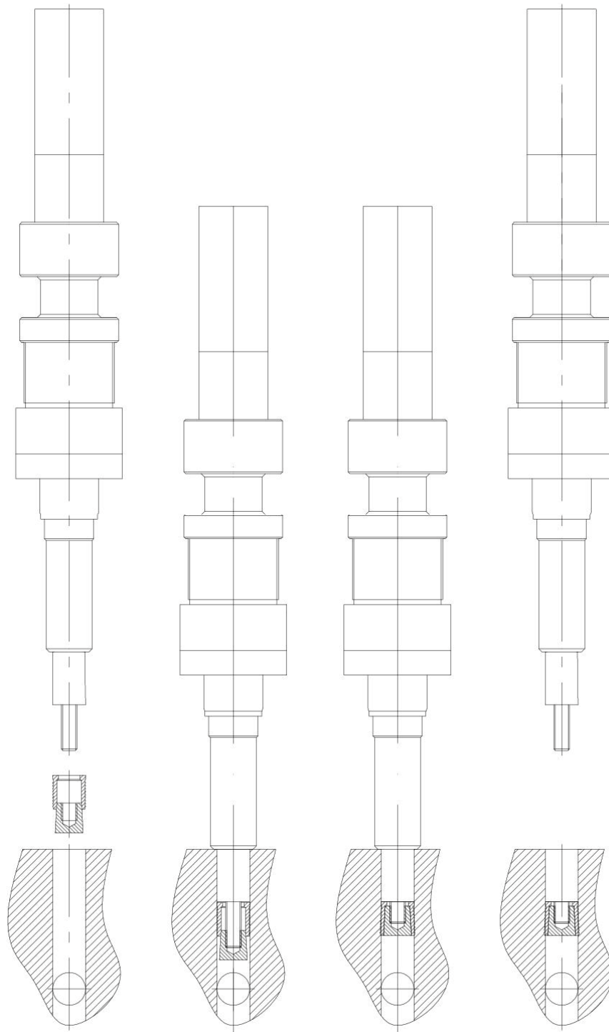
Threaded plugs
