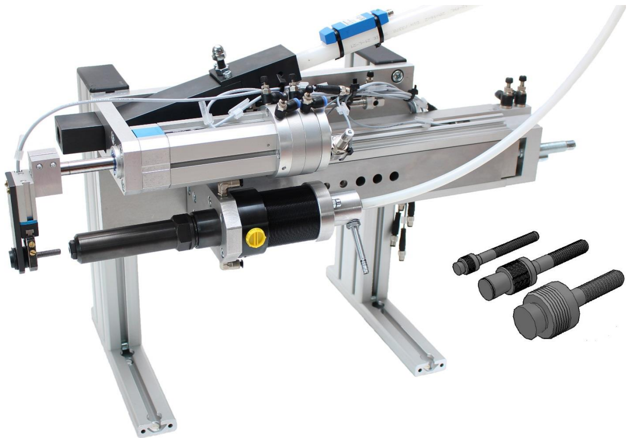
Rivet tool, automatic transfer and linear unit
